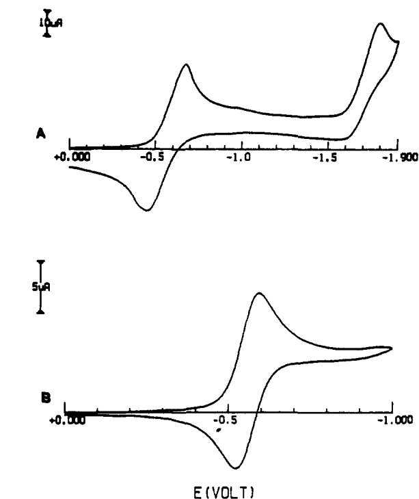
Figure 1. Cyclic voltammograms recorded at a mercury electrode on a deaerated tetrahydrofuran solution containing 1 ( 1.61 \times 10^{-3} mol dm -3 ) and (NBu 4 )(ClO 4 ) (0.2 mol dm -3 ) at a scan rate of (A) 0.2 and (B) 0.02 V s -1 .
