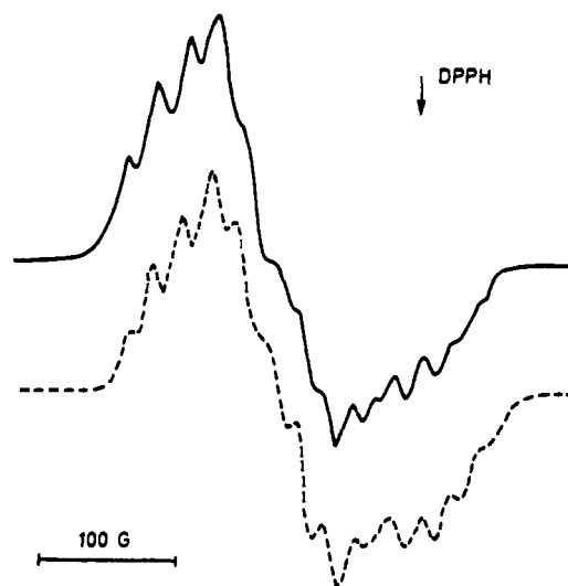
Figure 6. Experimental (full line) and computed (dashed line) X-band ESR spectra at 100 K of 11 dissolved in 2-methyltetrahydrofuran.
